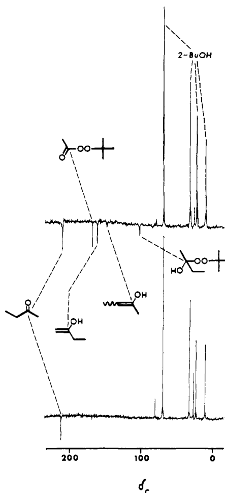
Figure 3. Carbon-13 spectra recorded during photolysis of t -BuOOH in 2-butanol ( 1H ). The top spectrum clearly shows two enolic signals. The bottom spectrum was of the same reaction but with 10^{-4} M p -toluenesulfonic acid added. Starting t -BuOOH concentration was 5% (v/v).
