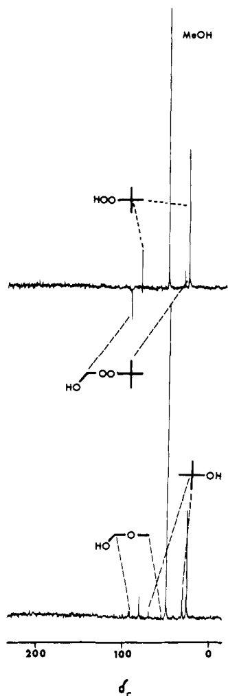
Figure 1. Carbon-13 spectra recorded during (top) and after (bottom) photolysis of t -BuOOH in methanol (1A). Starting concentration of the t -BuOOH was 10% (v/v).
