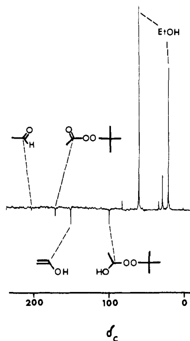
Figure 2. Carbon-13 spectrum recorded during photolysis of t -BuOOH in ethanol (1B). Starting concentration of t -BuOOH was 10% (v/v).
